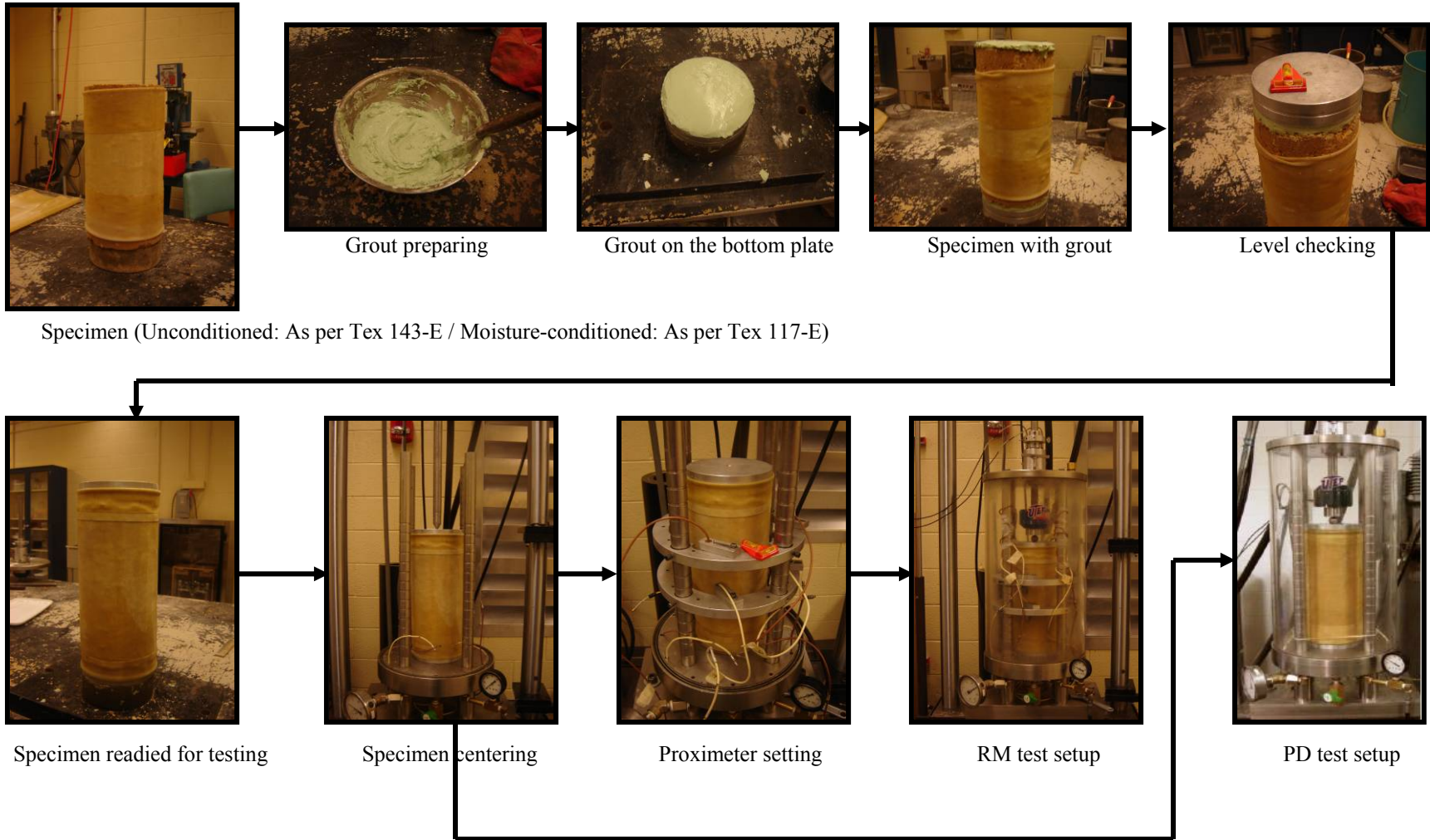
Figure 3.3 - Procedure for Repeated Load Triaxial Test
