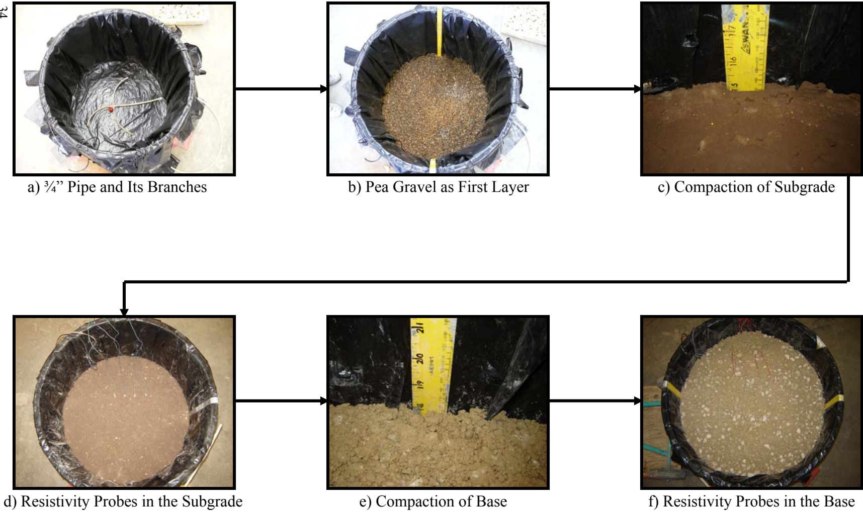
Figure 3.12 - Different Steps of Filling Tank
