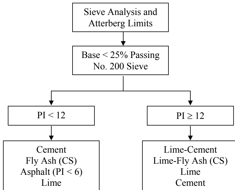
Figure 6.2 – Decision Tree for Selecting Type of Additive
