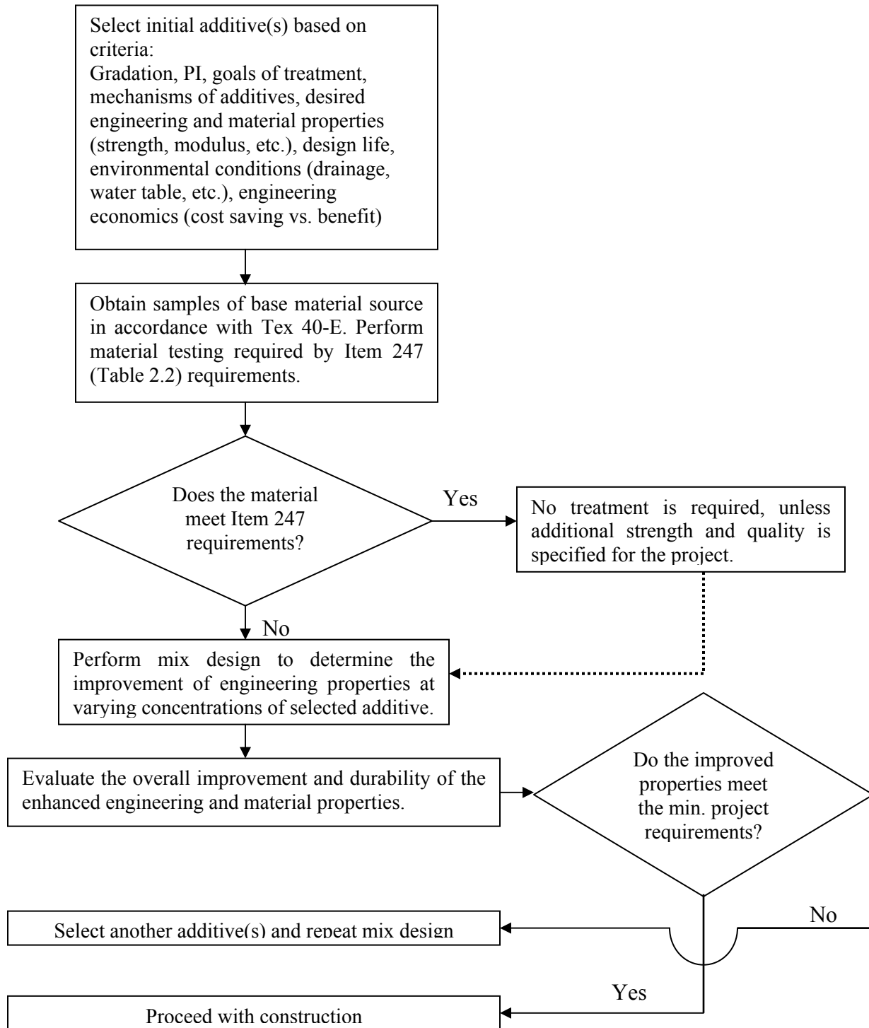
Figure 2.3 - Flowchart for Base Treatment (TxDOT, 2005)
