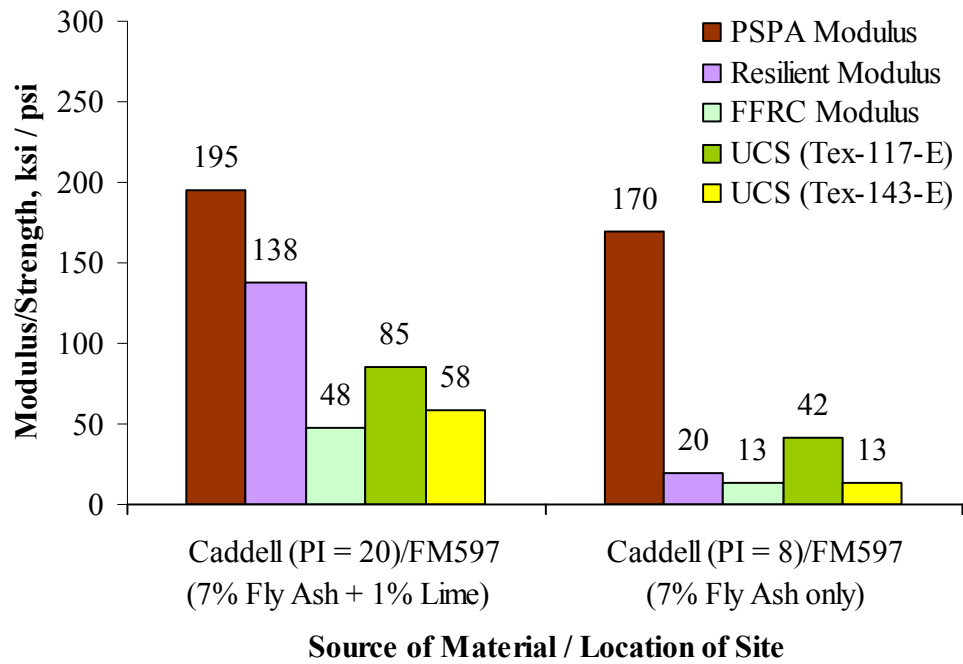
Figure 4.13 – Comparison of Results from PSPA Measurements and Laboratory Tests
