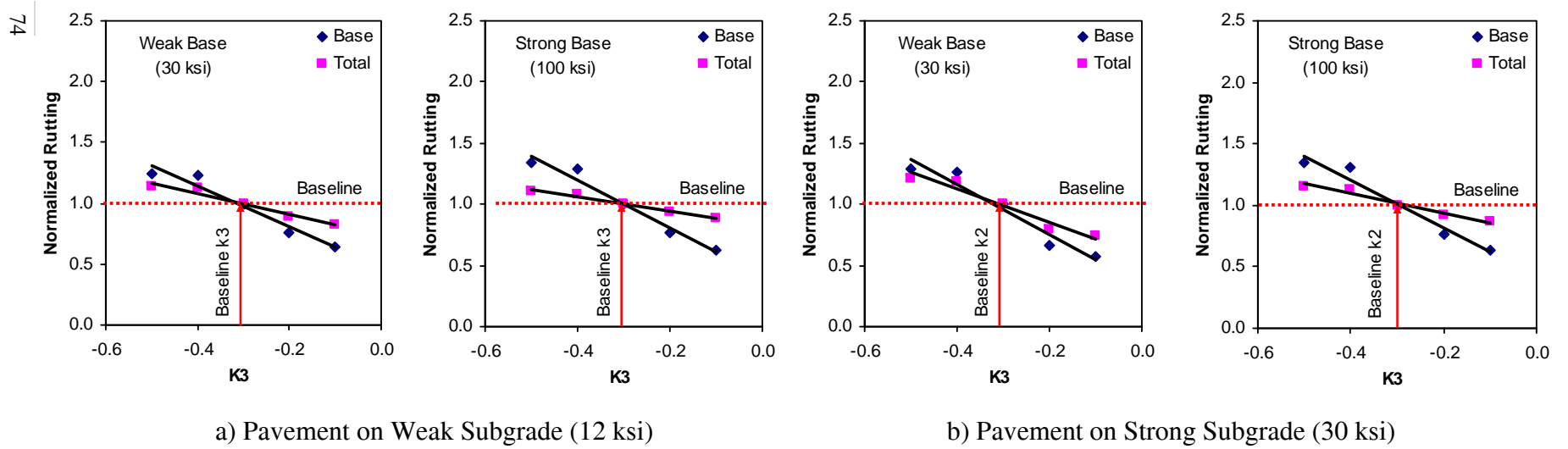
Figure 5.7 - Variations in Rutting with Parameter k_3 of Base
