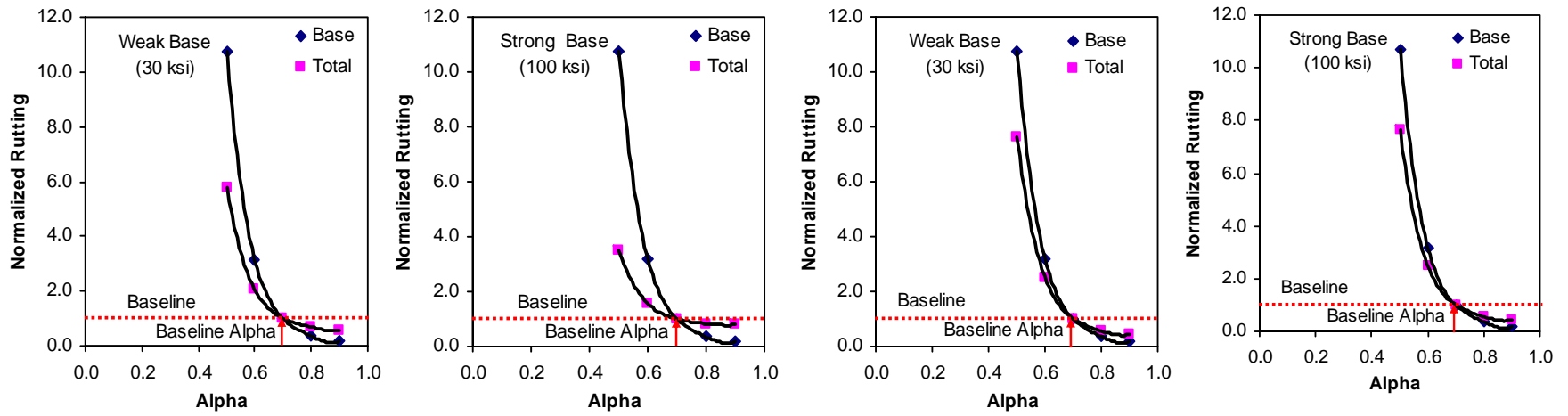
a) Pavement on Weak Subgrade (12 ksi)
