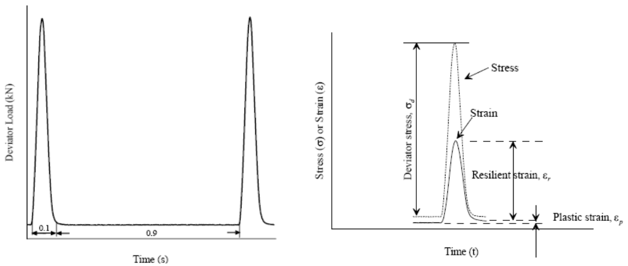
Figure 3.5 – Stress and Strain of One Load Cycle
