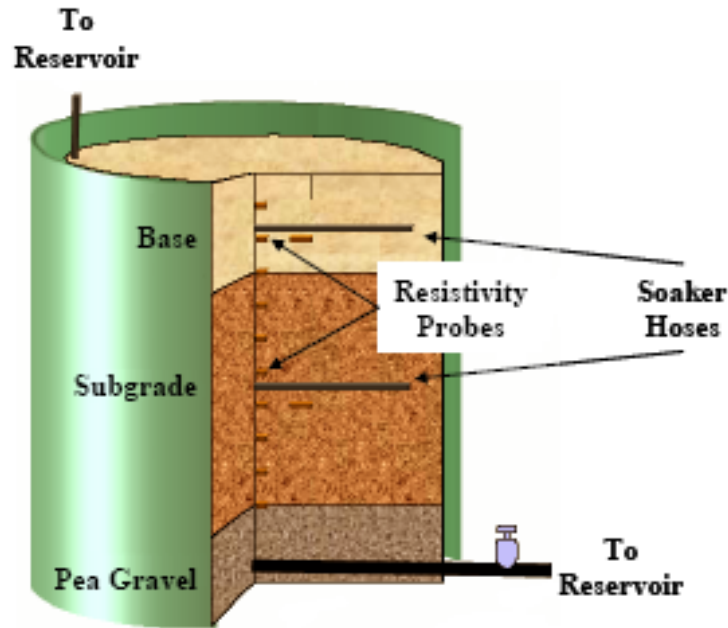
Figure 3.11 - Schematic Picture of Tank (Amiri, 2004)
