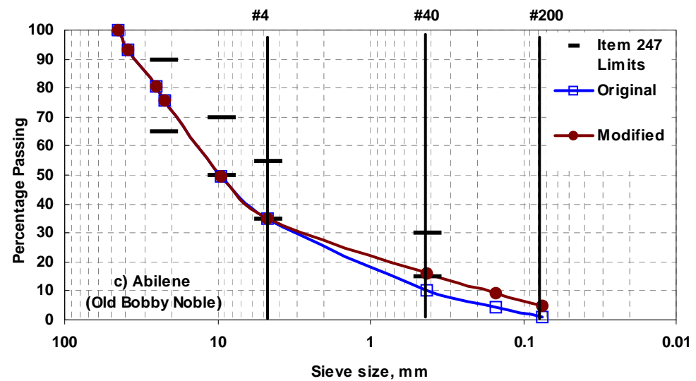
Figure 4.3 - Gradation Curves of Materials before and after Gradation Modification
