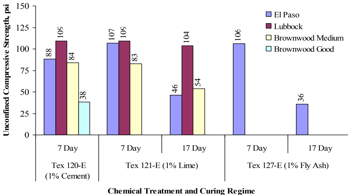
Figure 4.4 - Unconfined Compressive Strengths of Different Materials as per Tex 120-E, Tex 121-E and Tex 127-E
