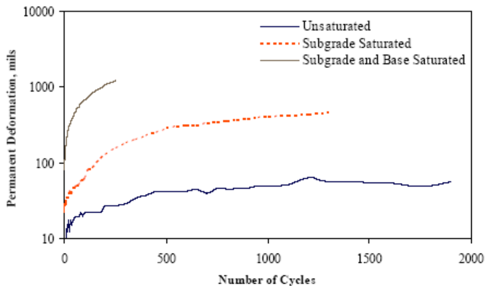
Figure 2.4 - Variations of Rutting with Number of Load Cycles
