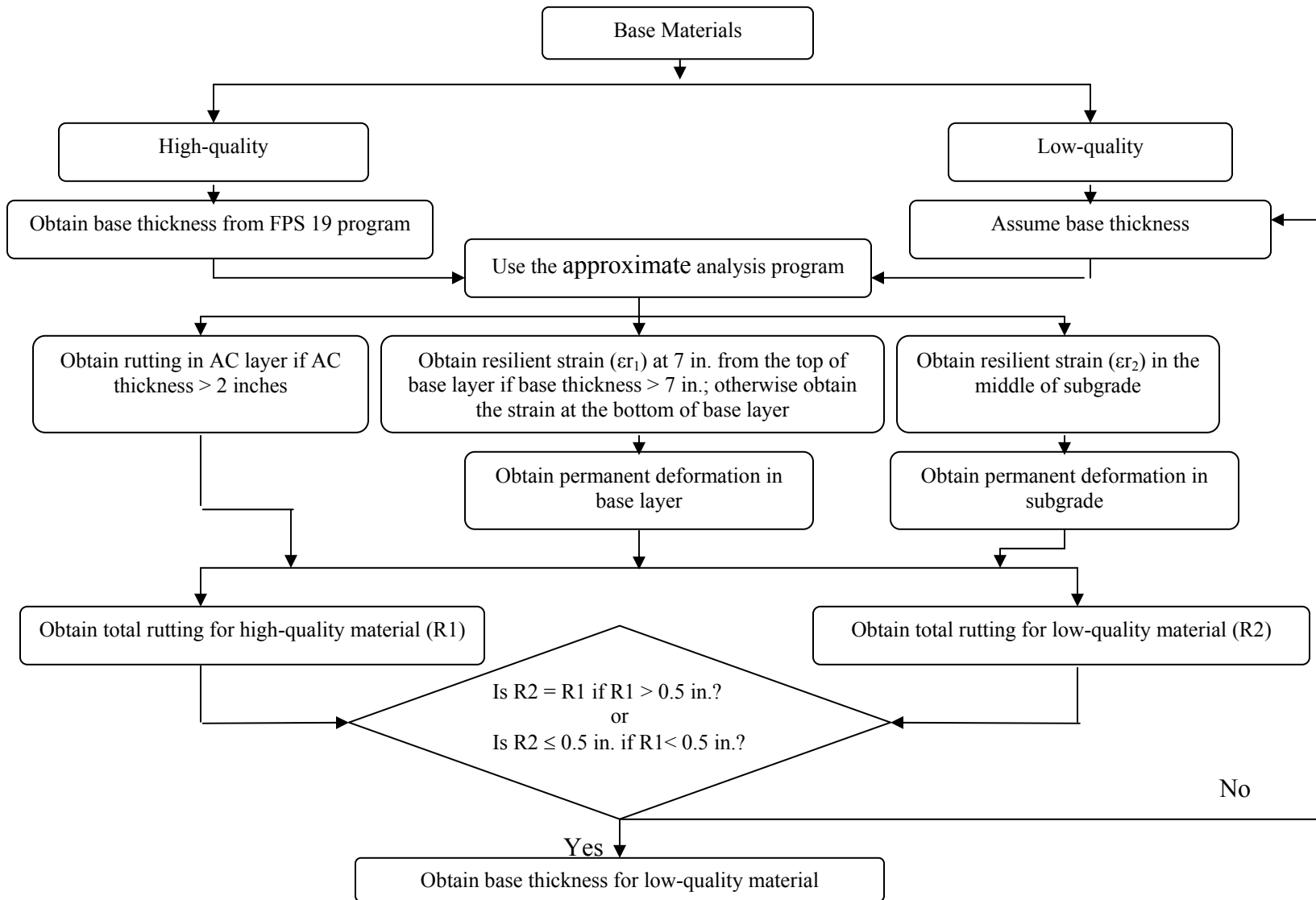
Figure 5.15 - Flow Chart for Determining Equivalent Base Thickness
