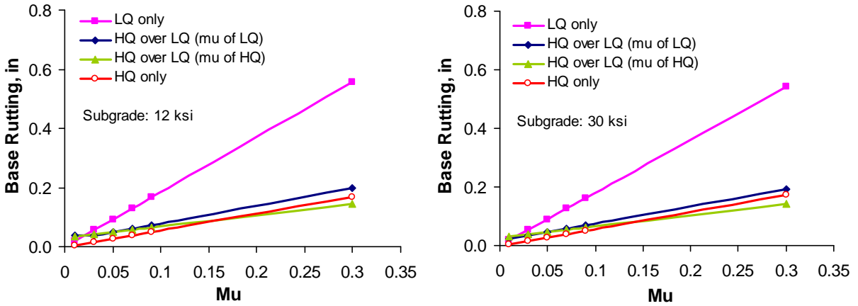
Figure 5.12 - Comparison of Variations in Rutting with Parameter Mu for Base Courses Consisting of One Layer and Two Layers
