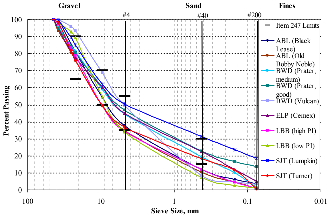
Figure 4.1 - Gradation Curves from Different Base Materials
