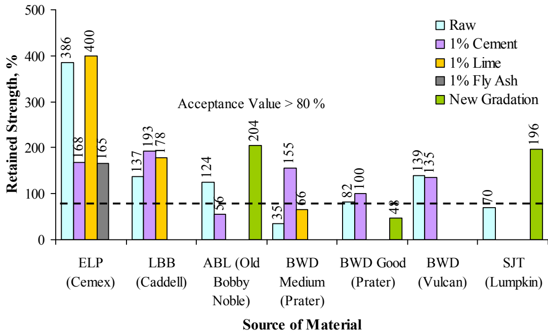
Figure 4.10 - Retained Strength of Different Materials
