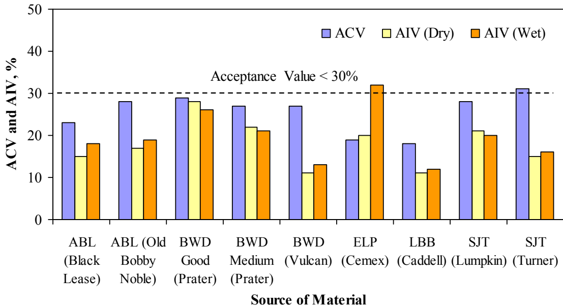
Figure 4.5 - ACV and AIV of Different Materials
