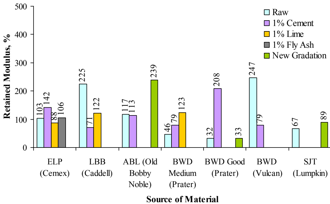
Figure 4.9 - Retained Moduli of Different Materials
