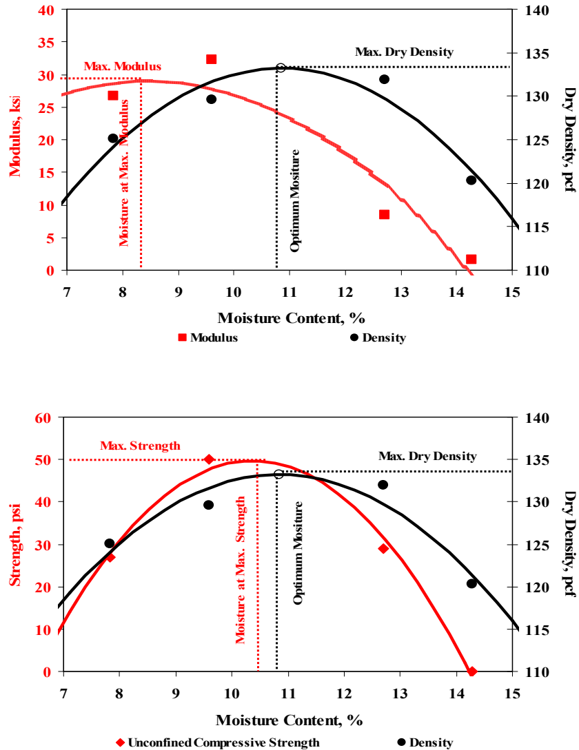
Figure 3.1 - Relationships between Moisture Content, Dry Density, Modulus and Strength
