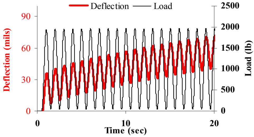
Figure 3.16 – Typical Pattern and Corresponding Deflections for Sinusoidal Loading
