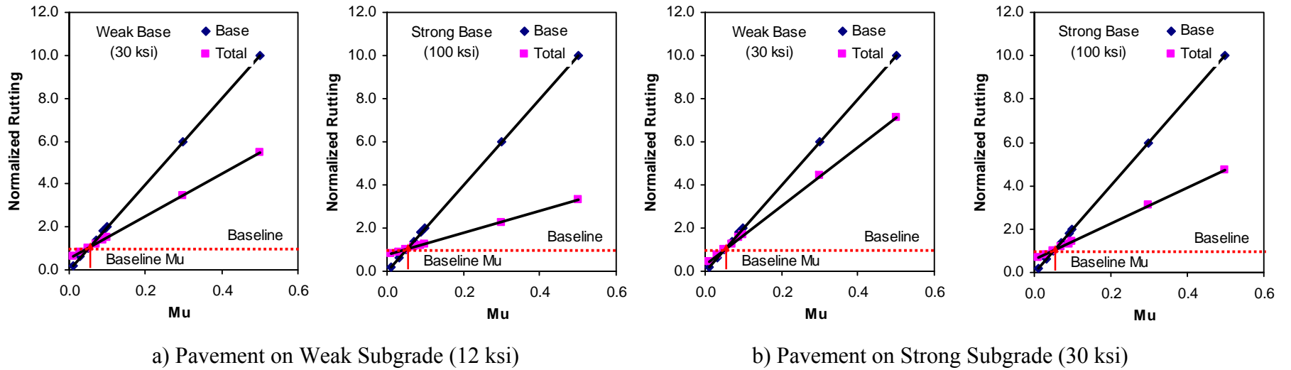
Figure 5.8 - Variations in Rutting with Parameter \mu of Base
