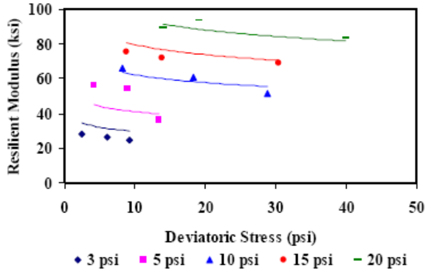
Figure 3.6 - Typical Result Obtained from Resilient Modulus Test
