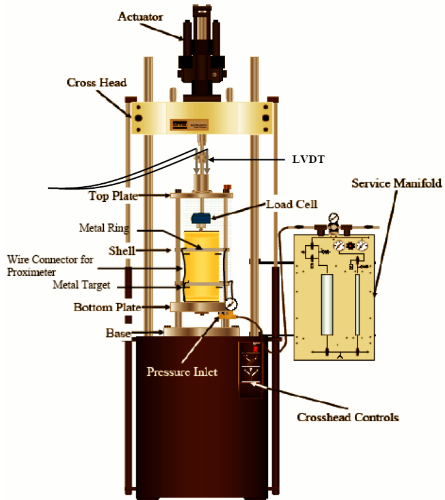
Figure 3.4 - Repeated Load Triaxial Load Schematic
