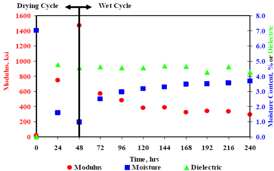
Figure 3.10 - Typical Variation in Modulus, Moisture and Dielectric Constant with Time
