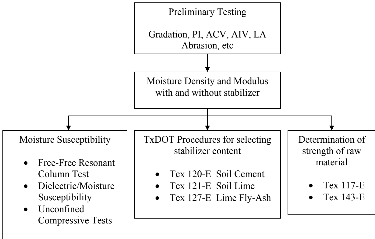
Figure 2.2 - Test Protocol for Characterizing Base Materials (Geiger et al., 2006)
