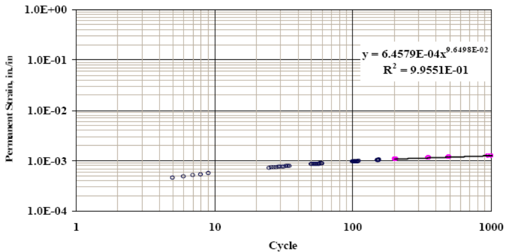
Figure 3.7 -Typical Result Obtained from Permanent Deformation Test
