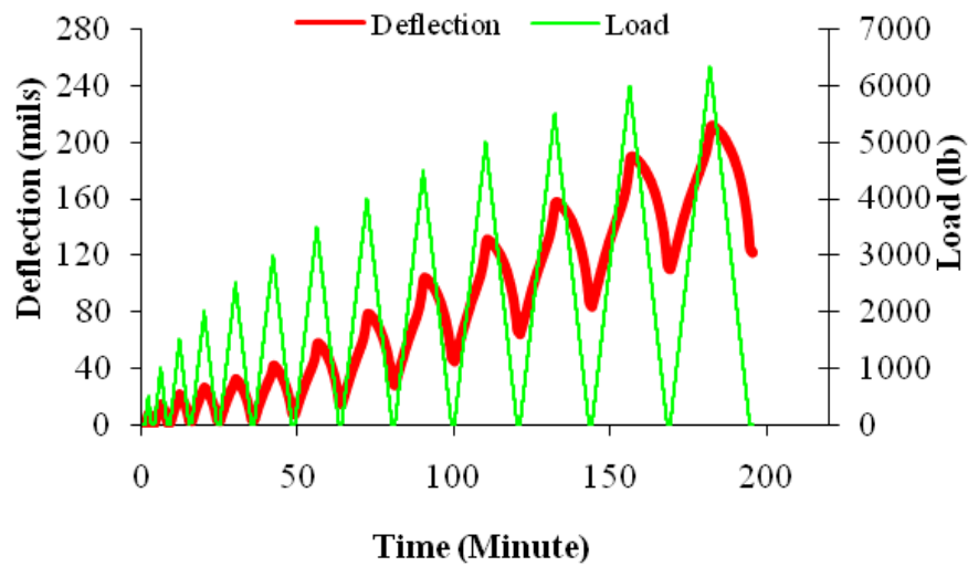
Figure 3.15 - Typical Pattern and Corresponding Deflections for Cyclic Ramp Loading
